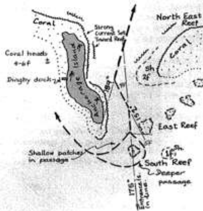
Detail of Approach and Anchorage
